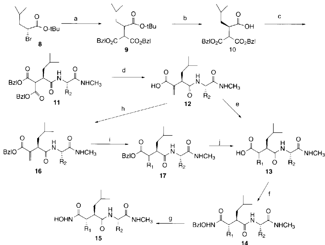
Scheme 2. The synthesis of hydroxamate inhibitors 15 . Reagents and conditions: (a) Dibenzyl malonate, t\text{BuOK} , DMF; (b) \text{HCOOH} ; (c) \text{H}_2\text{NCHR}_2\text{CONHCH}_3 ( 7 ), WSC, DMF; (d) (i) \text{H}_2 , 10% Pd/C, or \text{HCOONH}_4 , 10% Pd/C, MeOH; (ii) \text{HCHO} , piperidine; (e) nucleophile or \text{H}_2 , 10% Pd/C; (f) \text{H}_2\text{NOBzl} , HOBT, WSC, DMF; (g) \text{H}_2 , 10% Pd/C; (h) benzyl bromide, \text{NaHCO}_3 , DMF; (i) amine; (j) \text{H}_2 , 10% Pd/C.
