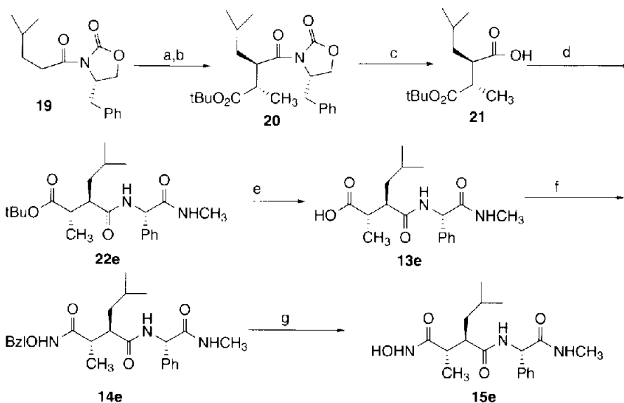
Scheme 3. The stereoselective synthesis of hydroxamate inhibitors 15e . Reagents and conditions: (a) (i) diisopropylamine, \text{BuLi} , THF; (ii) \text{CH}_3\text{CH}(\text{OSO}_2\text{CF}_3)\text{CO}_2\text{Bzl} ; (b) (i) \text{H}_2 , 10% Pd/C; (ii) isobutene, \text{H}_2\text{SO}_4 ; (c) 30% \text{H}_2\text{O}_2 , \text{LiOH} ; (d) \text{H}_2\text{NCH(Ph)CONHCH}_3 , WSC, DMF; (e) \text{HCOOH} ; (f) \text{H}_2\text{NOBzl} , HOBT, WSC, DMF; (g) \text{H}_2 , 10% Pd/C.
